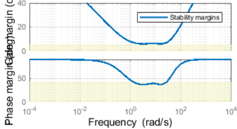
Requirement 3: Stability margins
