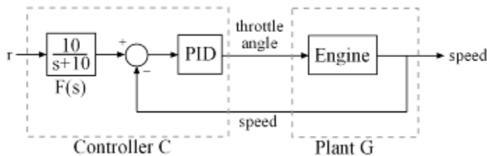
Figure 3: Feedback Loop for Engine Speed Control
