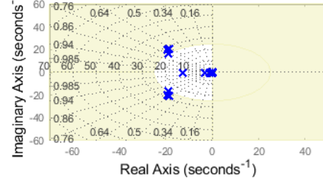
Requirement 4: Closed-loop pole location
