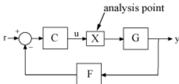
Figure 2: Analysis Point Block
