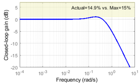
Requirement 2: Overshoot as a peak gain constraint
