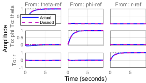
Requirement 1: Target response to step command
